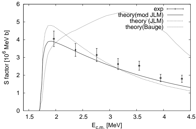
FIG. 6: Astrophysical S factor as function of proton energy for the reaction {}^{76}\text{Ge}(p,n){}^{76}\text{As} . Experimental S factors measured in this work are compared to NON-SMOKER calculations using the optical potentials of [35, 36] (JLM), of [38] (Bauge), and a modified JLM potential with an increased imaginary strength (see text).
