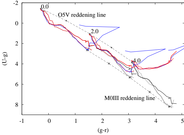
Figure B2. The synthetic colours of main-sequence stars, giants and supergiants including the effect of the U -band filter red leak plotted in the (U - g) vs. (g - r) colour-colour diagram. The colour-colour diagram without the effect of the U -band red leak was already shown in G09 (Fig.6). In this graph the black lines are the old G09 colours, the overplotted lines are the new synthetic colours of main-sequence stars (thick red), giants (blue) and supergiants (thin red) for E(B-V)=0.0, 2.0 and 4.0 using the reddening law of Cardelli et al. (1989). The upper and lower envelope curves (dashed) are the old O5V-reddening curve and the M0III-reddening curve of G09. Late M-giants from M7III to M10III, not shown in G09, were add.
