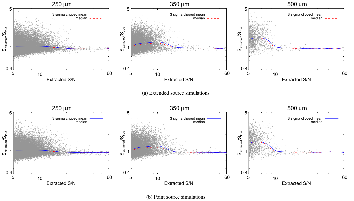
Figure 9. The ratio of flux densities for the matched sources in the simulated input (true) and extracted catalogues as a function of extracted signal to noise (S/N) for the three bands from the ESS and PSS maps. Also shown are the median and 3\sigma clipped mean values, calculated in bins of 0.05 in \log(S/N) .
