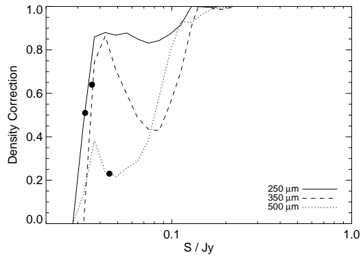
(b) The surface density correction required at each band to correct for the catalogue incompleteness, determined from the ratio of the flux-corrected to simulated input differential source counts. The solid dots indicate the position of the average 5\sigma limit in each band.
