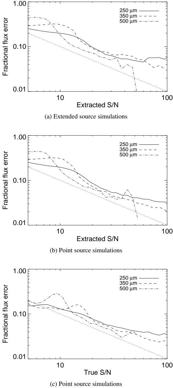
Figure 14. The fractional flux density error for the corrected extracted catalogues, ignoring any sources that fall outside the 99.73rd percentiles. The dotted lines indicate the expected behaviour.
