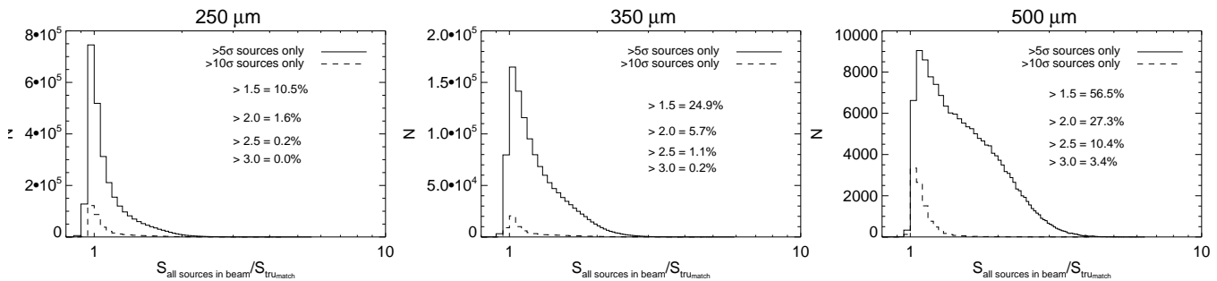
Figure 13. The PSF-weighted, background-subtracted, ratio of the sum of simulated input (true) sources within a beam to the flux density of the matched true source for > 5\sigma (solid line), and > 10\sigma (dashed line) sources in the extracted catalogue. The labels on the Figures give the percentage of sources with ratios greater than some particular value. The small proportion of sources where the ratio falls below 1 are due to the PSF-weighting.
