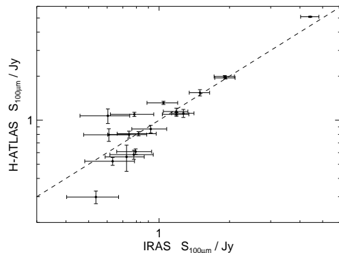
Figure 5. A comparison between the 100 \mu\text{m} flux densities from PACS and IRAS
