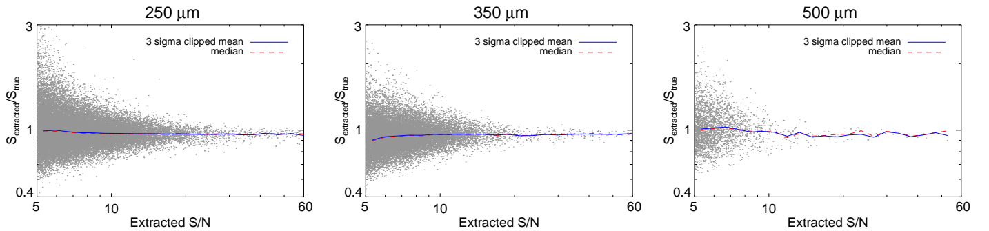
Figure 11. The ratio of flux densities for the matched sources in the simulated input (true) and extracted catalogues as a function of extracted signal to noise for the three bands, using the gridded position simulations (including point sources only). Also shown are the median and 3\sigma clipped mean values, calculated in bins of 0.05 in \log(S/N) . Note that confusion noise is not included in these simulations.
