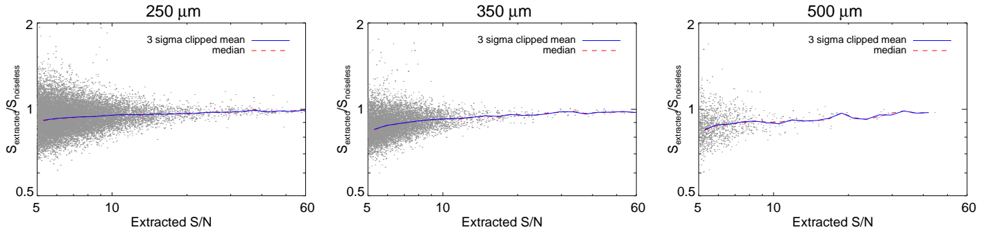
Figure 10. The ratio of flux densities for the matched sources in the noiseless MADX ( S_{\text{noiseless}} ) and extracted catalogues as a function of extracted signal to noise for the three bands (including point sources only). Also shown are the median and 3\sigma clipped mean values, calculated in bins of 0.05 in \log(S/N) .
