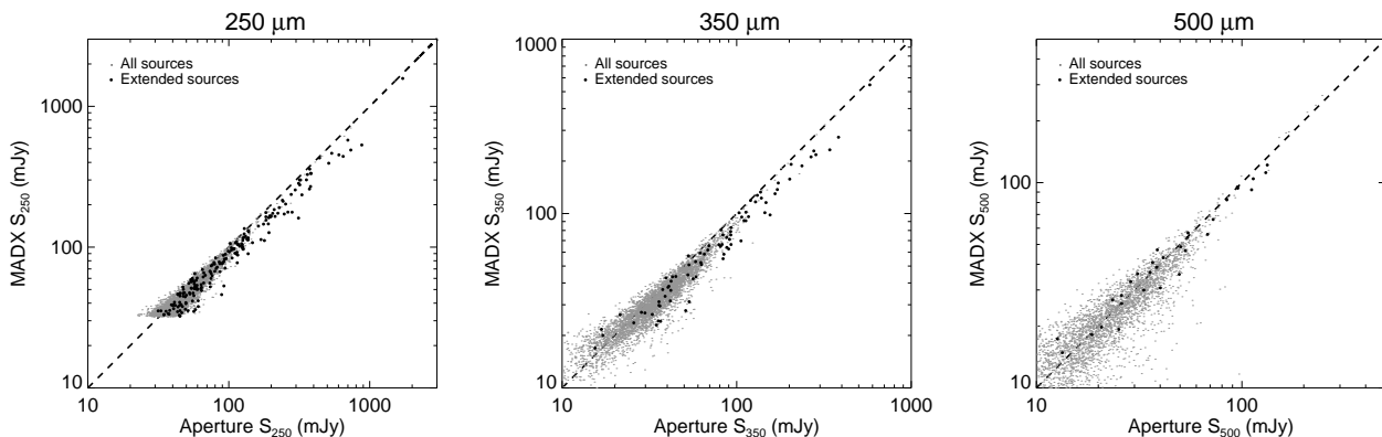
Figure 3. A comparison between the MADX and aperture measured fluxes for the sources with a possible optical identification in the matched catalogue of Smith et al. (2011). Source identified as extended are highlighted in bold.
