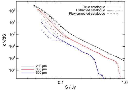
(a) The differential source counts for the extracted, simulated input (true) and flux-corrected catalogues for the three bands. Note the discrepancy between the flux-corrected and simulated input catalogues at faint flux densities.
