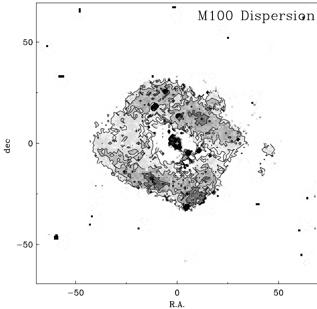
Fig. 4. Map of the velocity dispersion in H \alpha of the central part of the NGC 4321. The contours are situated at 20, 35, 50 and 65 km s ^{-1} .
