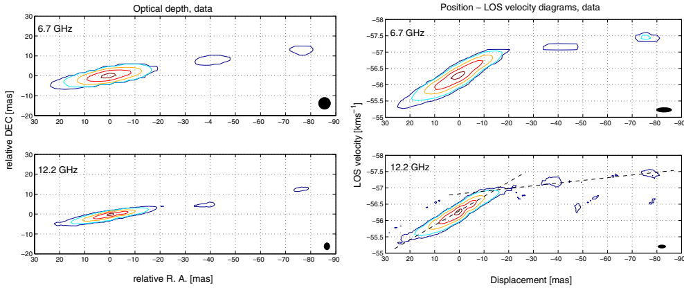
Figure 4. Maps (left) and velocity-displacement diagrams (right) of the main spectral feature of the 6.7 and 12.2 GHz methanol masers toward NGC7538 IRS 1. The beam size is shown in the bottom right corner in all panels. The contours are 1, 5, 10, 30, 50, 70, 90% of the peak in all panels. Dashed lines indicate the change in gradient between the main feature and the outliers.
