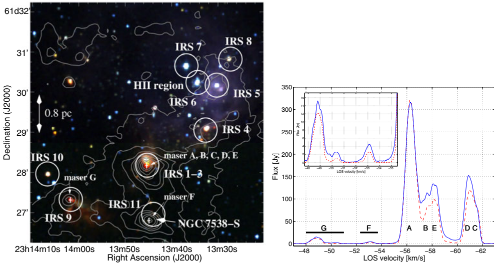
Figure 3. Left: General view of the high-mass star forming region NGC7538. Grey contours of the 1.2 mm dust continuum are overlaid on a JHK 2-mass image. Circles indicate the catalogued IR sources, crosses the methanol masers. The methanol masers appear in association with the youngest and most massive objects. Right: Spectrum of the 6.7 GHz maser emission toward NGC7538. Features A, B, C, D, E are cospatial with IRS 1. The maser disc is feature A. The inset is a zoom of the features F and G. The 12.2 GHz spectrum is similar to the 6.7 GHz one.
