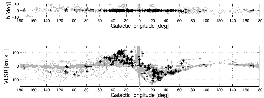
Figure 1. Distribution of methanol masers in Galaxy, superposed on the CO contours from Dame et al. 1987, in space (top) and LOS velocity (bottom). The methanol masers seem to accurately follow the overall structure of the Galaxy, both in space and LOS velocity. Particularly visible in the bottom panel is the fact that methanol masers are tracing the spiral arms ( 150^\circ > l > 80^\circ and -40^\circ > l > -90^\circ ) and the high rotational velocity of the nuclear ring ( l \approx 0^\circ ).
