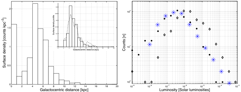
Figure 2. Left: Surface density of the known methanol masers in Galactocentric distance. The distribution shows a peak at the same radius as OB associations. The inset shows a comparison of the surface density of the masers with the molecular gas in the Milky Way. Right: Luminosity distribution of methanol masers in the Galaxy. Diamonds and circles plot all the (ambiguous) sources at the near- and far heliocentric distance, respectively. Stars show a synthetic luminosity distribution obtained by observing with a 2 Jy sensitivity a population of 5000 masers spatially distributed according to a Gaussian and having an intrinsic luminosity distribution as a power-law between cutoffs of index -1.7 .
