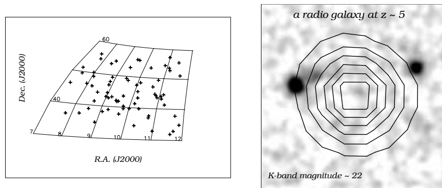
Figure 1. Left Location of all 6C** sources within the survey region. Right The 1.4 GHz radio contours overlaid onto a NIRI (Gemini) K-band image of a candidate z > 5 , 6C** radio galaxy. The image has a size of 14'' \times 18'' .
